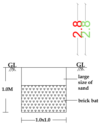
RAINWATER HARVESTING
