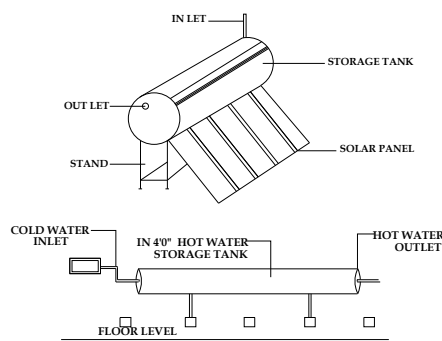
SOLAR HOT WATER SYSTEM DETAILS
