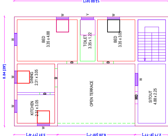
PRO. FIRST FLOOR PLAN. [NORTH FACING]
