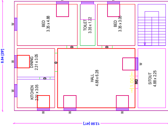
PRO. GROUND FLOOR PLAN. [NORTH FACING]
