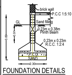
FOUNDATION DETAILS
