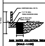
RAIN WATER COLLECTION TRENCH (SCALE-1:100)
