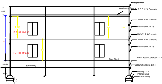
SECTION - AA Section
