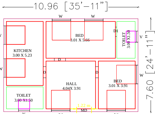
GROUND FLOOR (EAST FACING)
