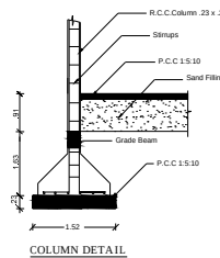
COLUMN DETAIL
