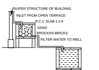
RAINWATER HARVESTING
