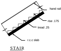
STAIR
