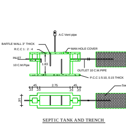
SEPTIC TANK AND TRENCH
