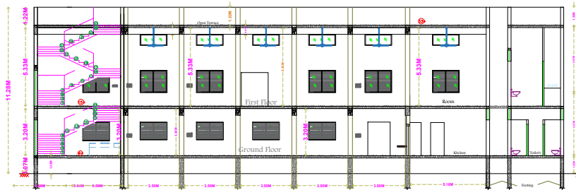
Sectional Details of AB
