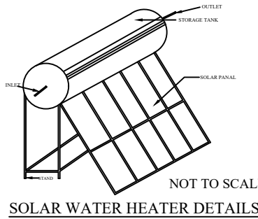
SOLAR WATER HEATER DETAILS NOT TO SCALE
