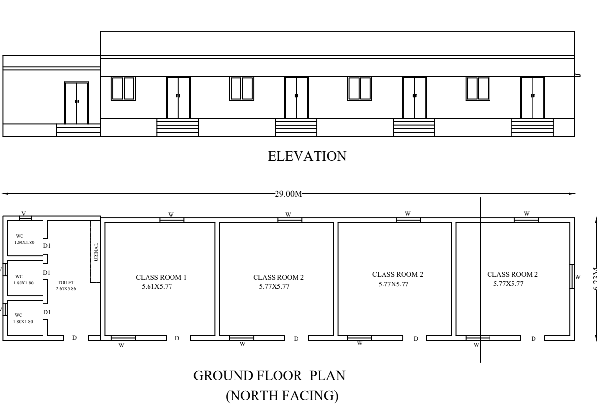
EXISTING BUILDING (BLOCK 2)
