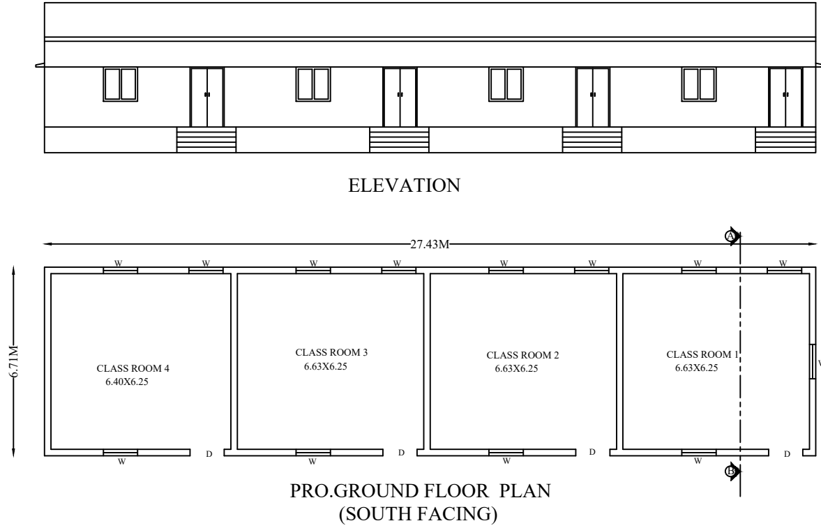
PROPOSED BUILDING (BLOCK 1)
