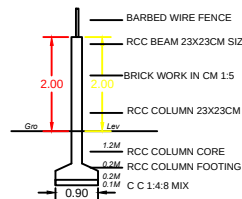
COMPOUND WALL DETAILS
