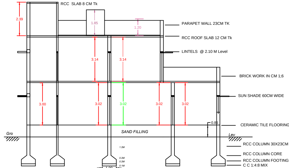
SECTIONAL ELEVATION ON X X' AXIS
