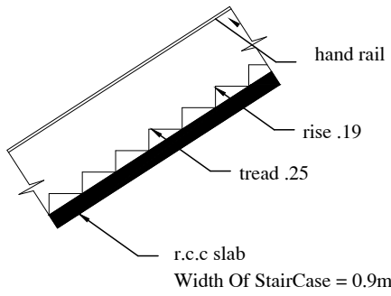
STAIRCASE DETAILS
