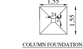
COLUMN FOUNDATION
