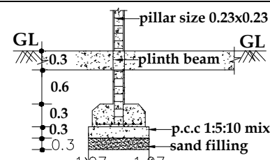
FOUNDATION DETAILS
