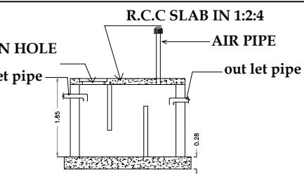
SEPTIC TANK SECTION
