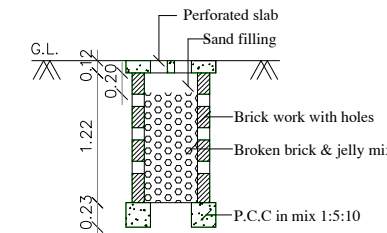
PERCOLATION PIT
