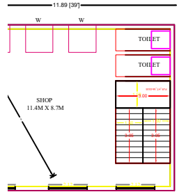
ED GROUND FLOOR PLAN
