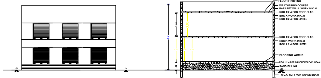
FRONT ELEVATION
