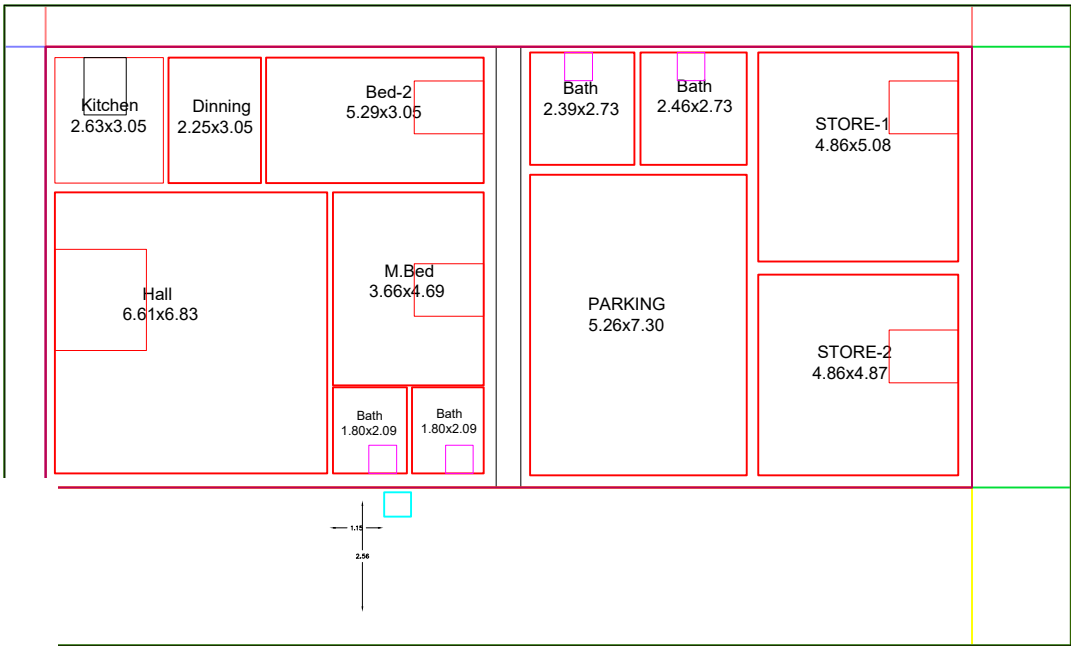
Ground Floor Plan (Faceing of North)
