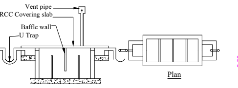
Septic Tank With U Trap Not To Scale
