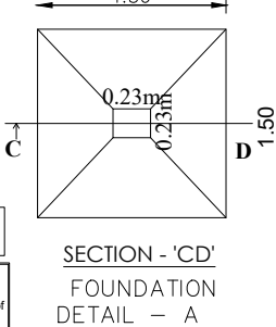
Isolated Footing -A (1.50X1.50) (Not to Scale)
