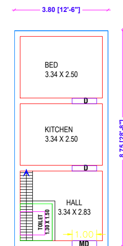
PRO. GROUND FLOOR PLAN. [EAST FACING]
