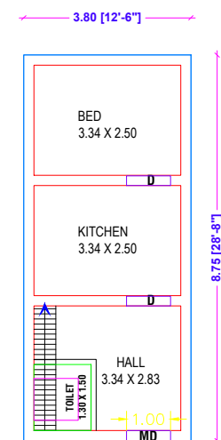
PRO. FIRST FLOOR PLAN. [EAST FACING]
