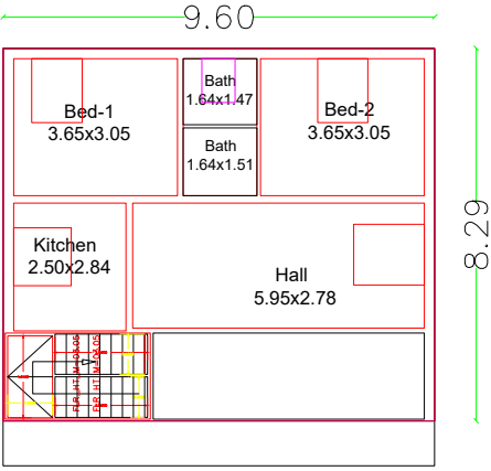
Proposed First Floor Plan (Facing of East)
