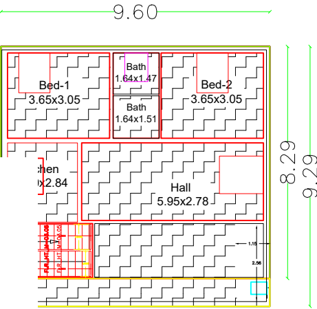
Existing Ground Floor Plan (Facing of East)
