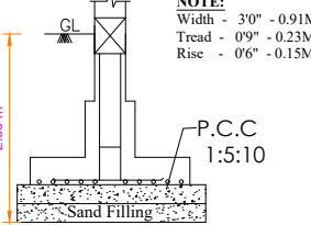
Isolated Footing -A (1.50X1.50) (Not to Scale)
