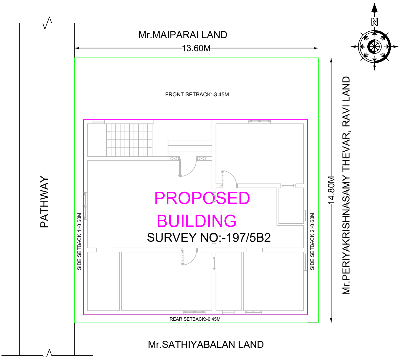
SITE PLAN
