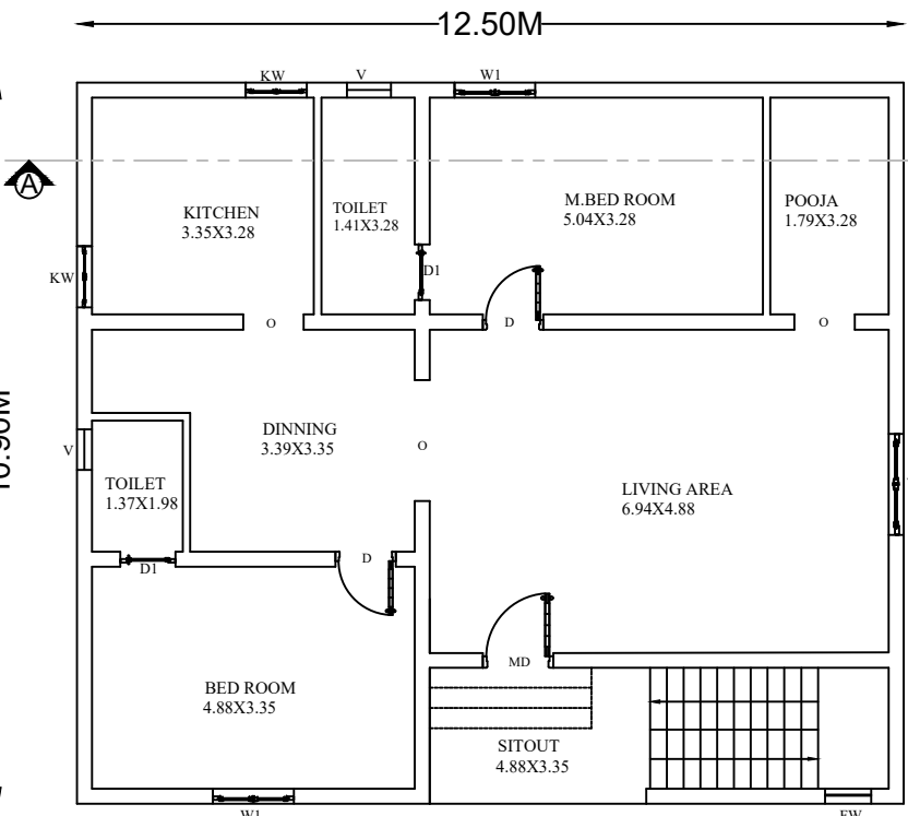
GROUND FLOOR PLAN (NORTH FACING)
