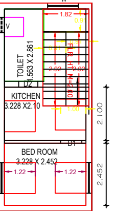
PRO. FIRST FLOOR PLAN.
