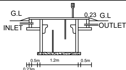
SEPTIC TANK DETAILS NOT TO SCALE
