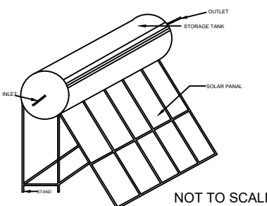
SOLAR WATER HEATER DETAILS NOT TO SCALE
