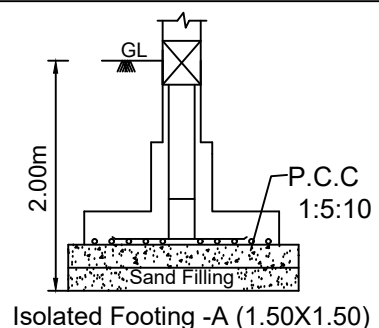
FOUNDATION DETAIL NOT TO SCALE
