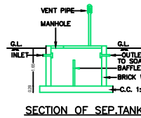
SECTION OF SEP.TANK
