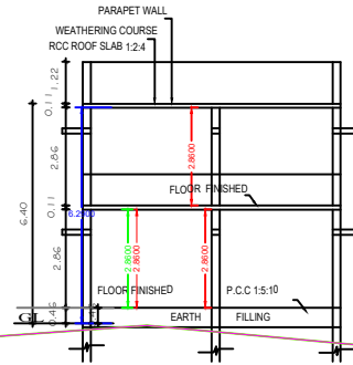
SECTION "A-B"
