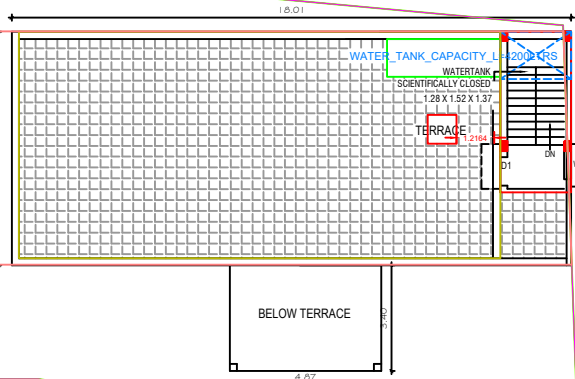
PRO. FIRST FLOOR TEARS PLAN.
