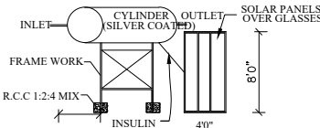
Waste Water Recycle Unit Not To Scale
