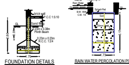
FOUNDATION DETAILS
