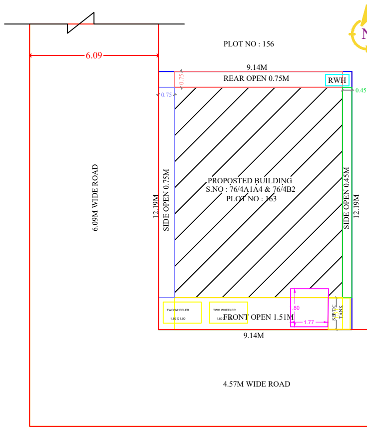
KEY PLAN
