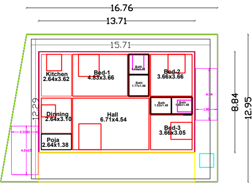
GROUND FLOOR PLAN FACING OF NORTH
