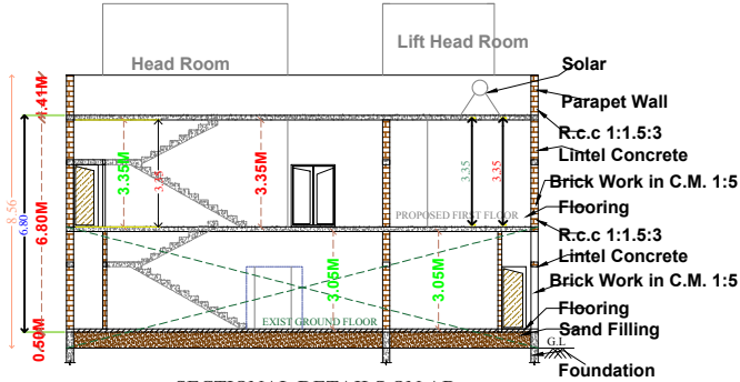
SECTIONAL DETAILS ON AB
