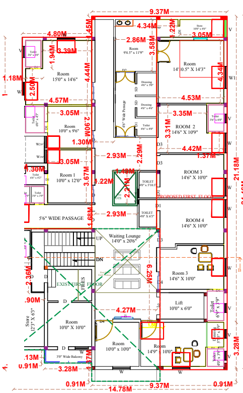
PART PROPOSED FIRST FLOOR PLAN
