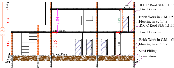
Sectional Details
