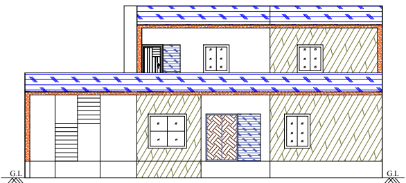
Elevational Details
