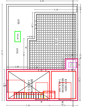
PROPOSED SECOND FLOOR PLAN
