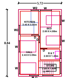
PROP. GROUND FLOOR PLAN (North Facing)
