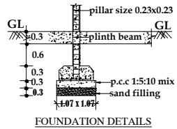
FOUNDATION DETAILS
