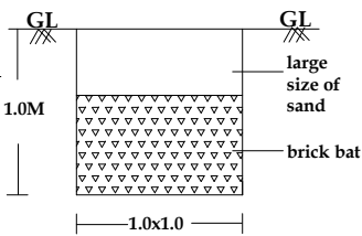
RAINWATER HARVESTING
