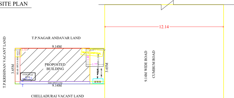
SITE PLAN
