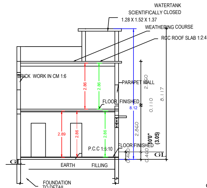
SECTION "A-B"
