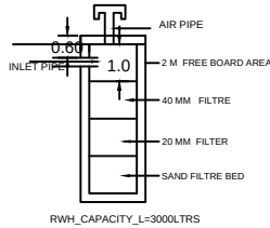
RWH_CAPACITY_L=3000LTRS
