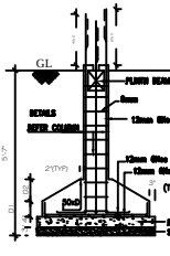
FOUNDATION DETAILS SCALE : 1:50.
