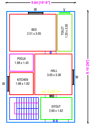
GROUND FLOOR PLAN [ EAST FACING ]
