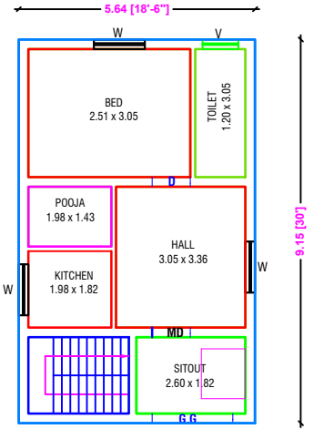
FIRST FLOOR PLAN [ EAST FACING ]
