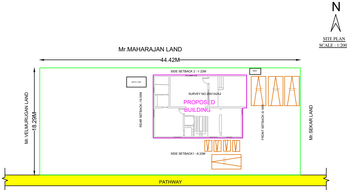
SITE PLAN
