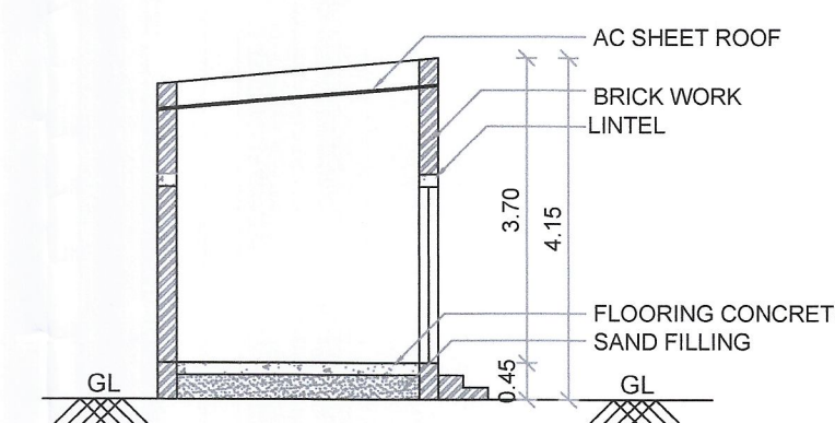
EXISTING BLOCK-4 SECTION - AA
