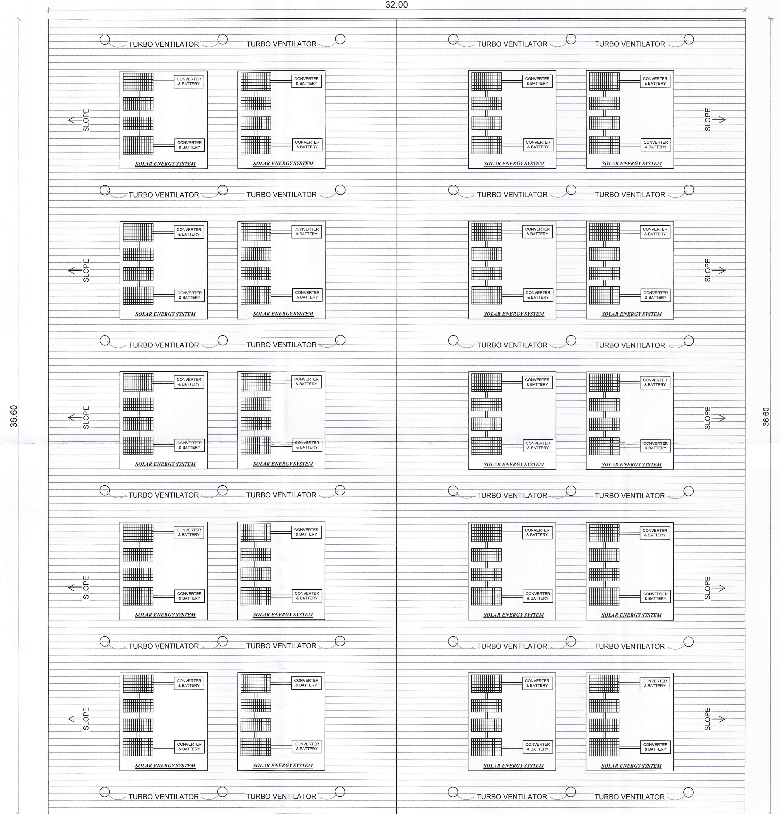
PROPOSED BLOCK - 1 TERRACE FLOOR PLAN
