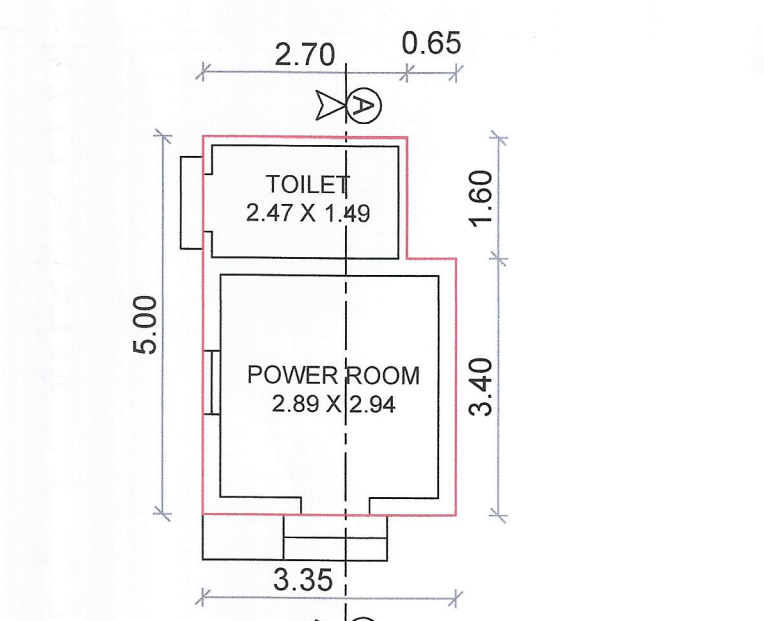
EXISTING BLOCK-3 GROUND FLOOR PLAN
