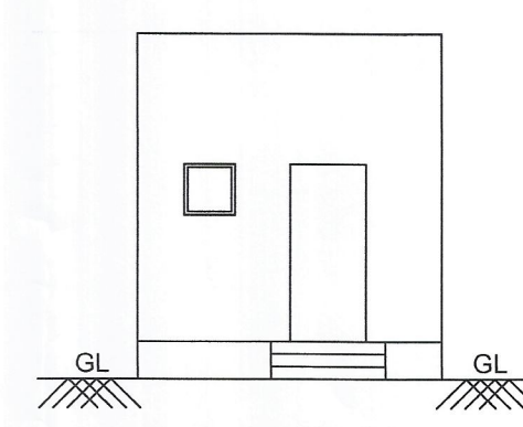
EXISTING BLOCK-4 ELEVATION
