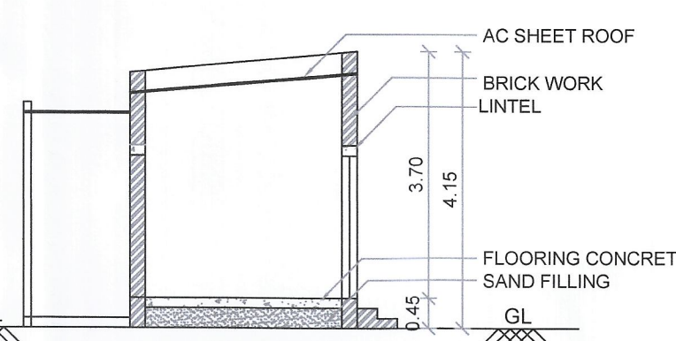
EXISTING BLOCK-3 SECTION - AA
