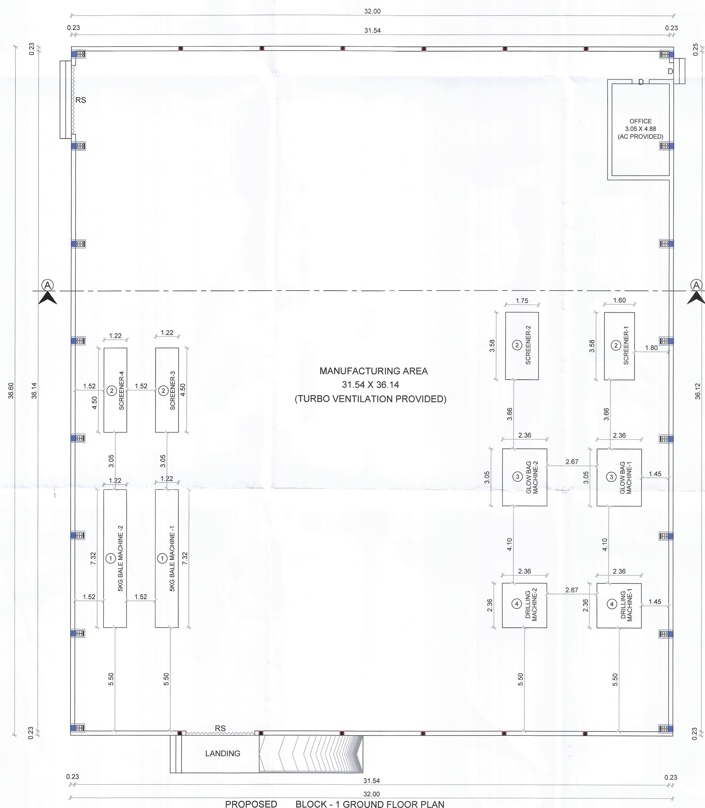
PROPOSED BLOCK - 1 GROUND FLOOR PLAN
