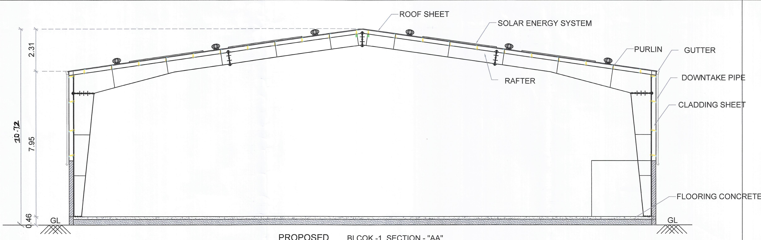
PROPOSED BLOCK-1 SECTION - "AA"
