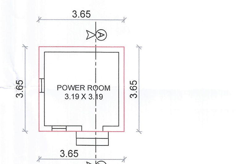
EXISTING BLOCK-4 GROUND FLOOR PLAN
