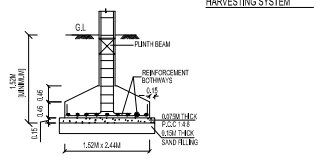
TYP. DET. COLUMN & FOUNDATION FOOTING
