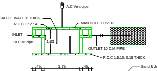
SEPTIC TANK AND TRENCH
