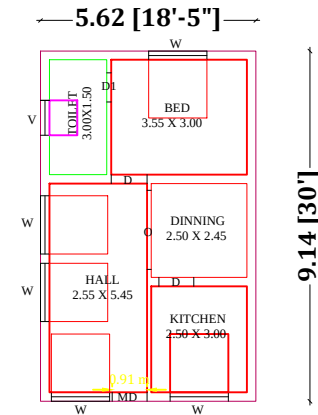
GROUND FLOOR PLAN SOUTH FACING
