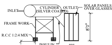
Waste Water Recycle Unit Not To Scale
