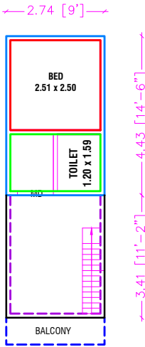
PRO. SECOND FLOOR PLAN [NORTH FACING]
