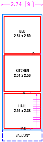
PRO. GROUND FLOOR PLAN [NORTH FACING]
