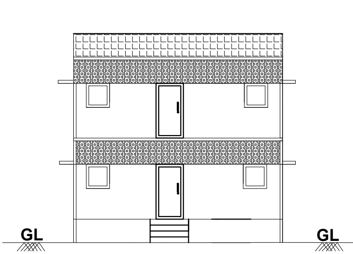
FRONT ELEVATION
