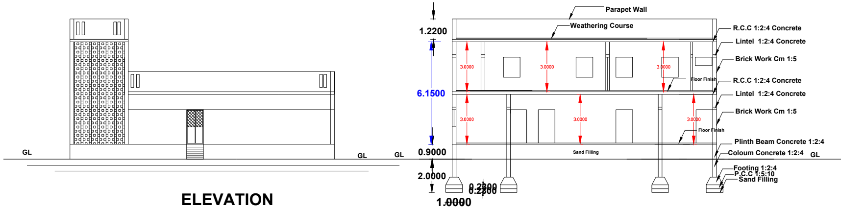
Section - AA
