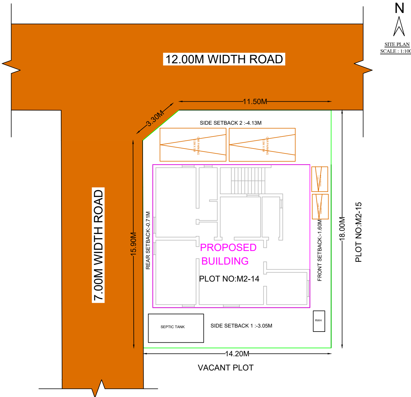
SITE PLAN
