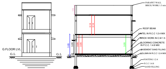
ELEVATION (South Facing)
