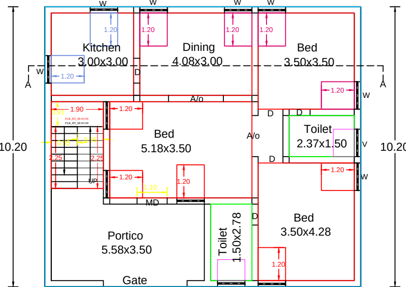
GROUND FLOOR PLAN (Facing North)
