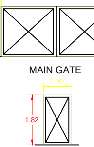
WICKET GATE
