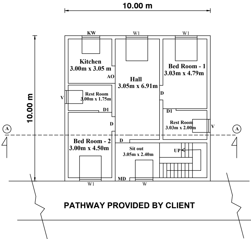
PROPOSED GROUND FLOOR PLAN ( NORTH FACING )
