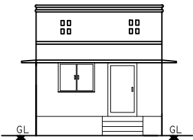
FRONT ELEVATION
