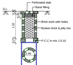
PERCOLATION PIT FOR 30sq.m. (Scale:- 1:50)
