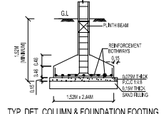
TYP. DET. COLUMN & FOUNDATION FOOTING
