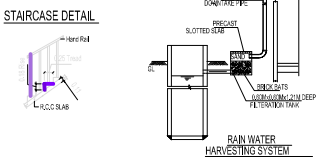
STAIRCASE DETAIL
