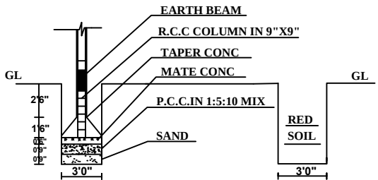
FOUNDATION DETAILS
