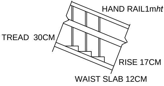
STAIRCASE DETAILS
