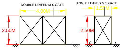
MAIN GATE DETAIL
