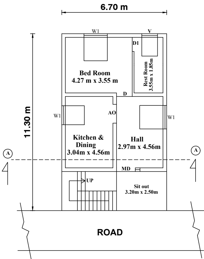
PRO. GROUND FLOOR PLAN EAST FACING
