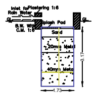
RAIN WATER PERCOLATION PIT
