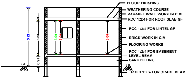
SECTION "A-B"
