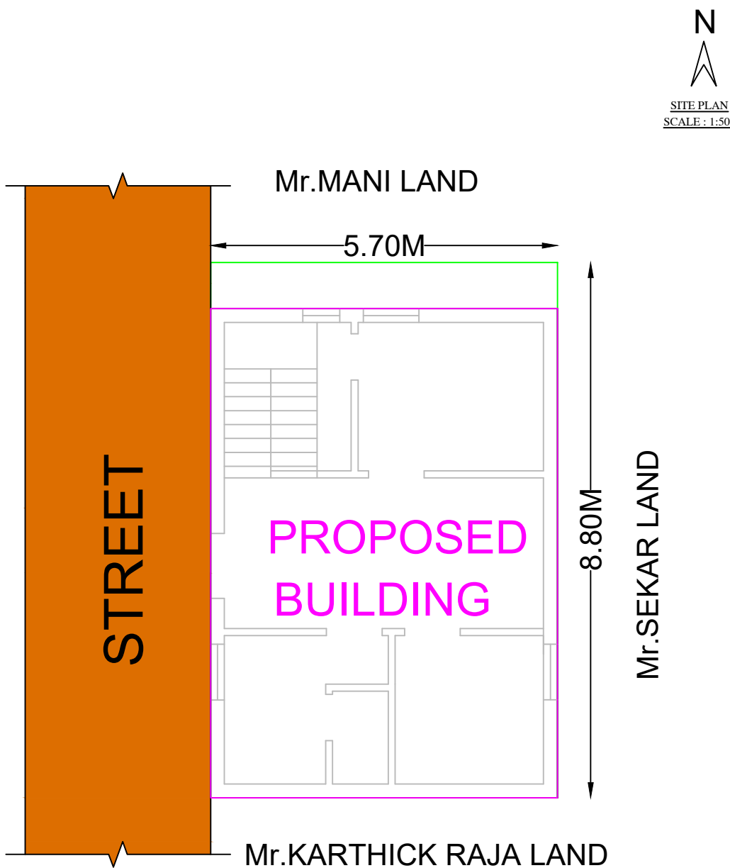
SITE PLAN
