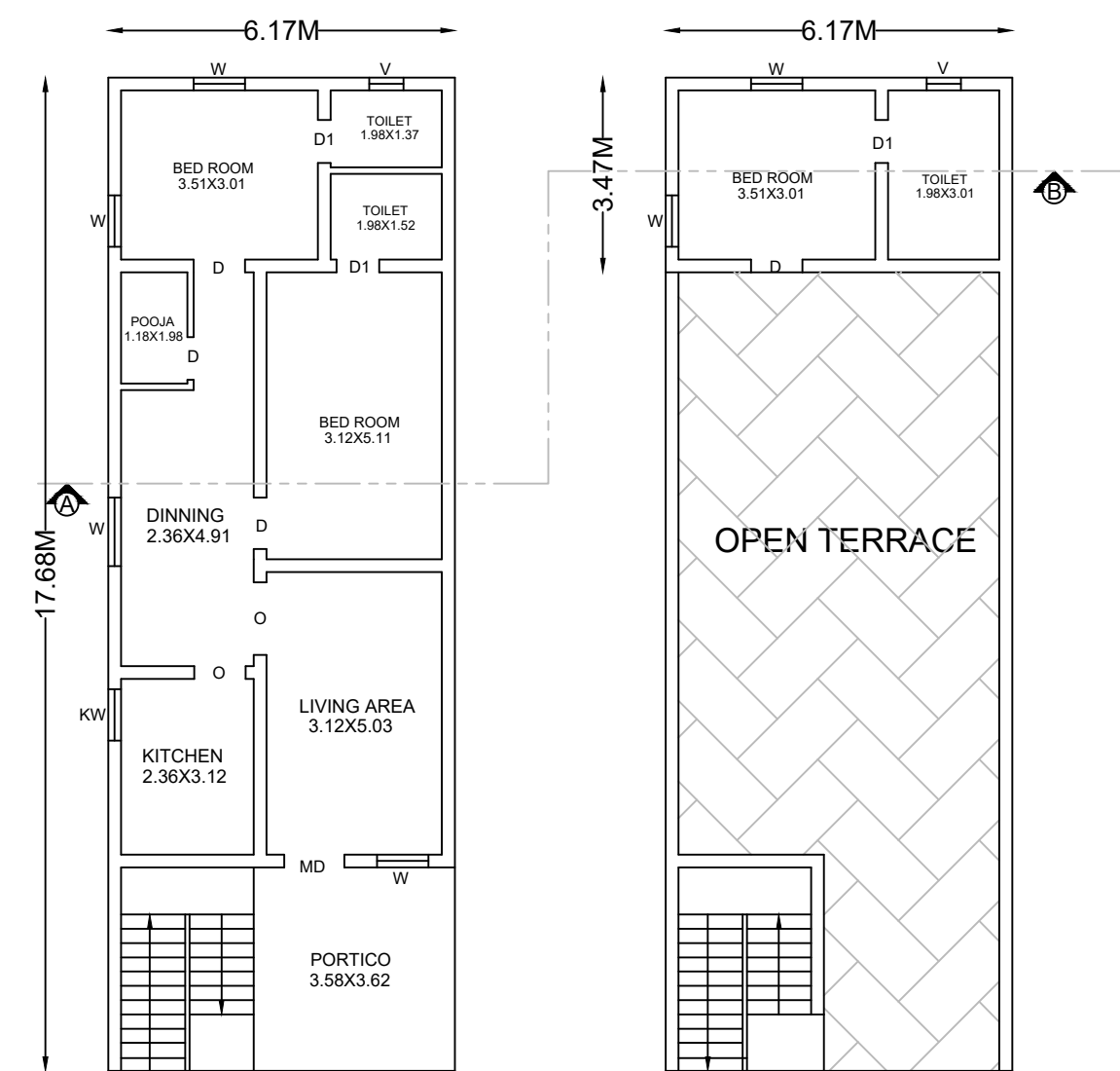
FIRST FLOOR PLAN (EAST FACING)
