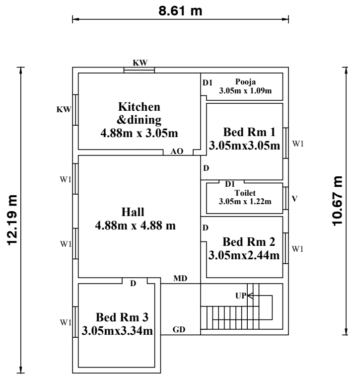
EXISTING GROUND FLOOR PLAN WEST BLOCK
