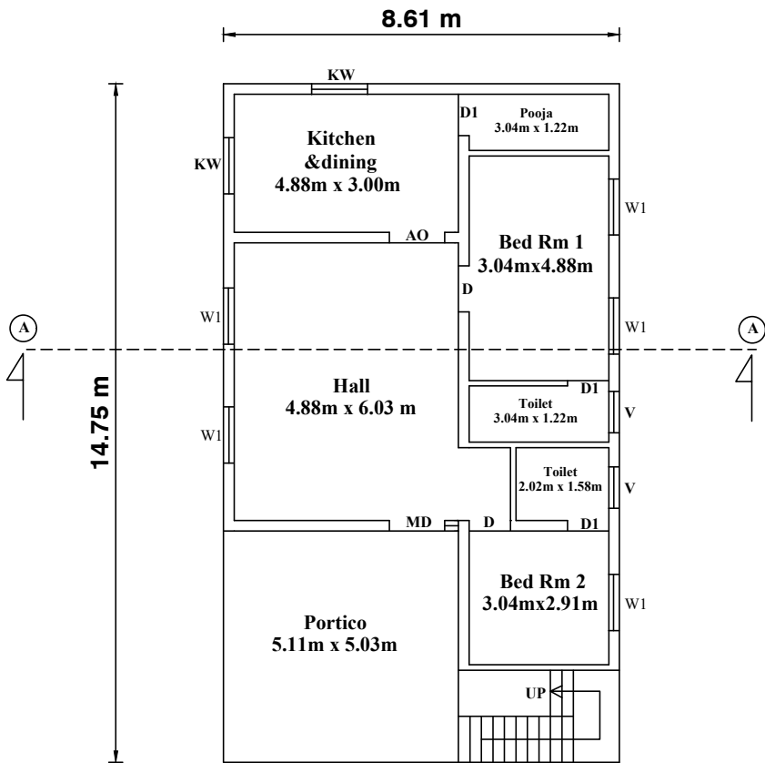
PRO . GROUND FLOOR PLAN EAST BLOCK
