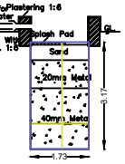
FOUNDATION DETAILS
