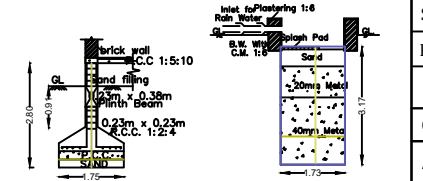
FOUNDATION DETAILS
