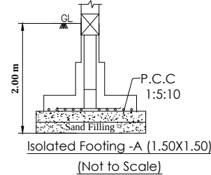
FOUNDATION DETAIL -
